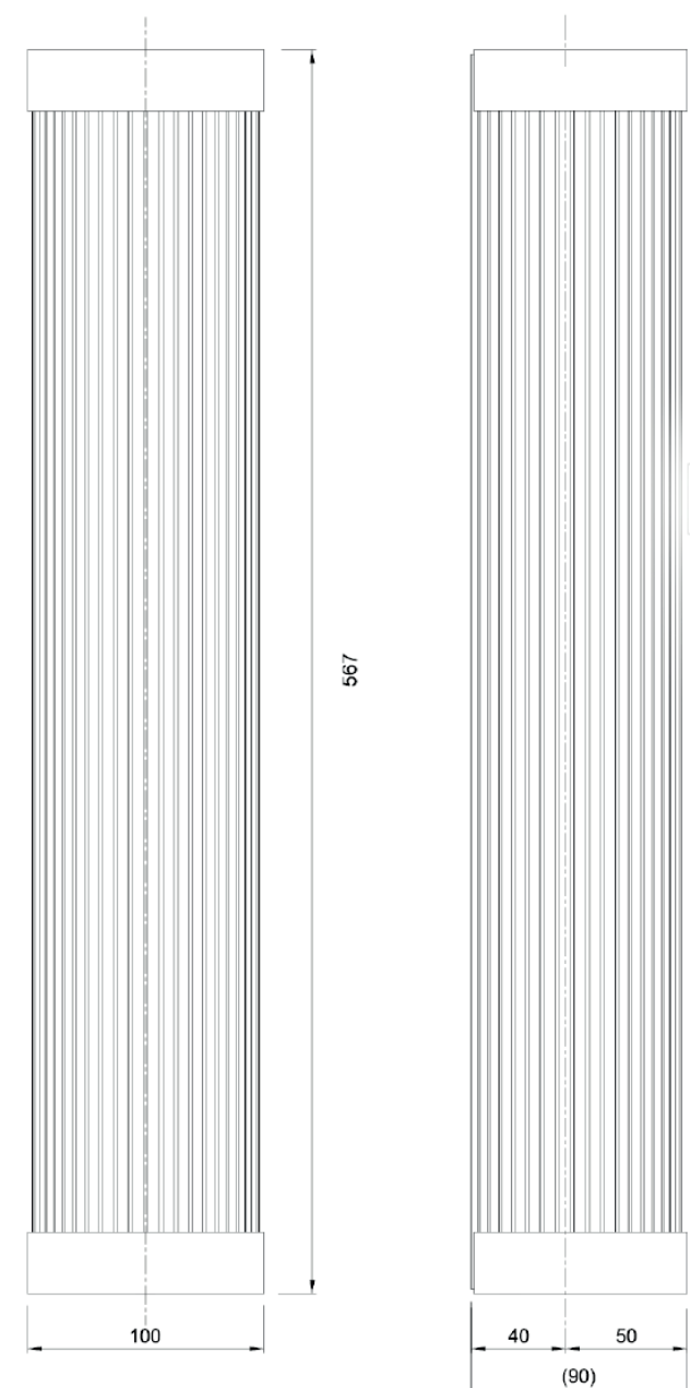
FRONT VIEW
