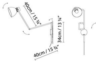
BLUX SYSTEM W40 PLUG-IN
