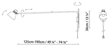
BLUX SYSTEM W125 PLUG-IN
