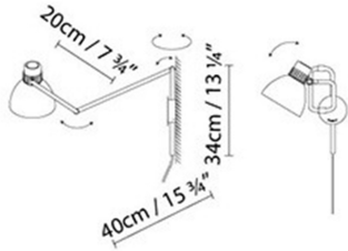
BLUX SYSTEM W20 PLUG-IN
